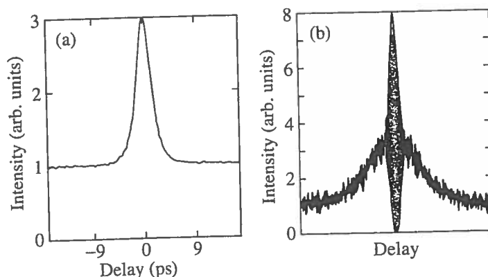
Figure 3.12 (a) Intensity autocorrelation and (b) interferometric autocorrelation for highly chirped pulses from a mode-locked Ti:S laser. A 2-ps pulse width and a time-bandwidth product \Delta\nu\Delta t = 2.7 are calculated assuming a \text{sech}^2 intensity profile. For (b), the delay axis is zoomed by roughly a factor of 3 compared to (a). From [52].
