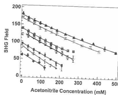
Figure 3. SHG electric field as a function of concentration of acetonitrile added to C314 solutions at varying bulk concentrations: 7.6 \mu\text{M} (red solid diamond), 8.5 \mu\text{M} (blue open diamond), 9 \mu\text{M} (dark red solid box), 10 \mu\text{M} (black open circle), 11.5 \mu\text{M} (dark green solid box), 12.7 \mu\text{M} (green open box) and 14 \mu\text{M} (dark blue solid triangle). Curves shown are the fit using eq 5.
